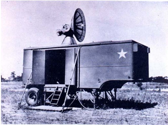
Exterior view of radio set SCR-584, a mobile radar unit. In: "AAF Manual 105-101-2 Radar Storm Detection," by Headquarters, Army Air Forces, August 1945. Courtesy of NOAA Photo Library.
