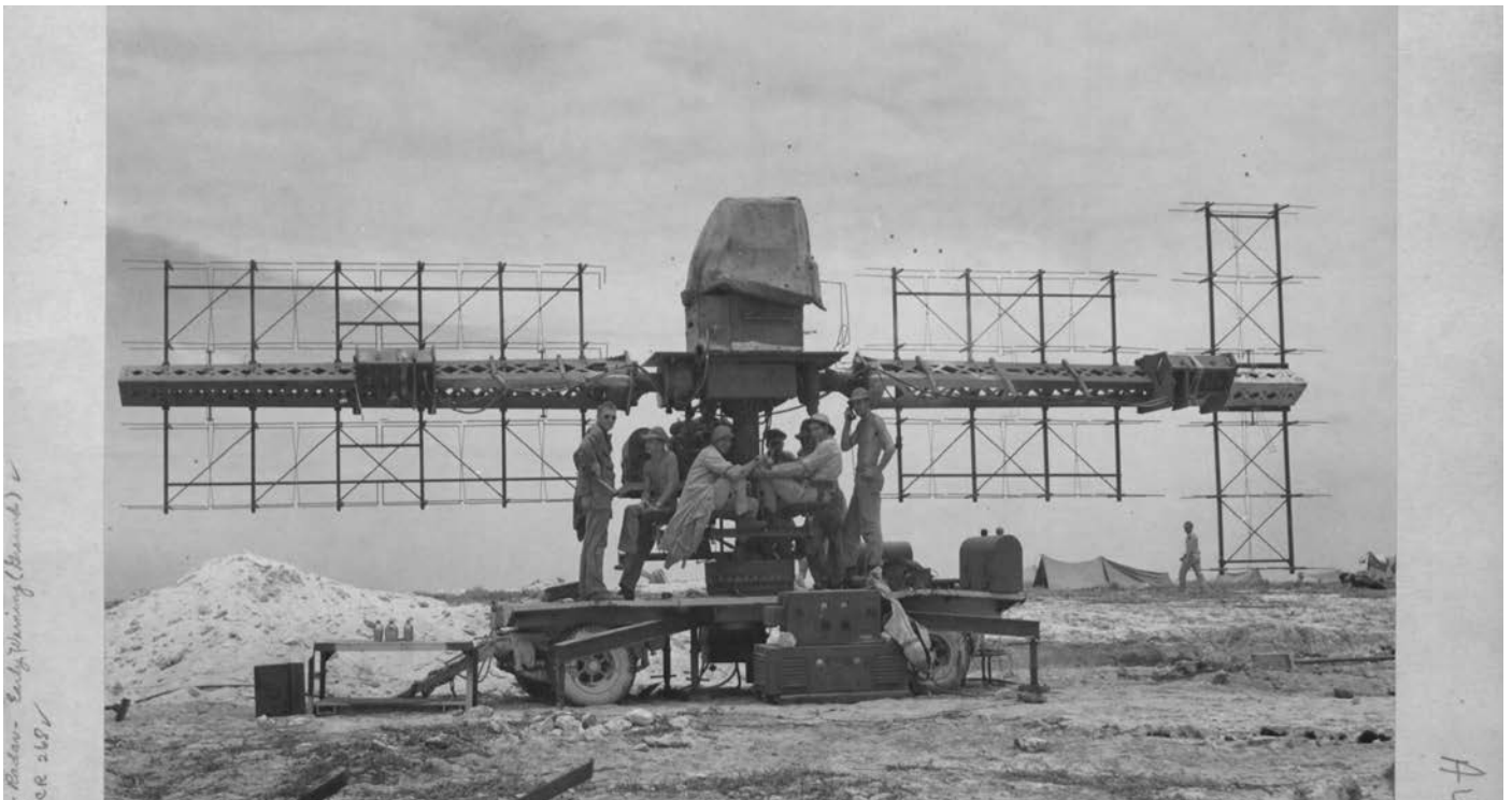
Image of a SCR-268 radar. Courtesy of the Library of Congress.
